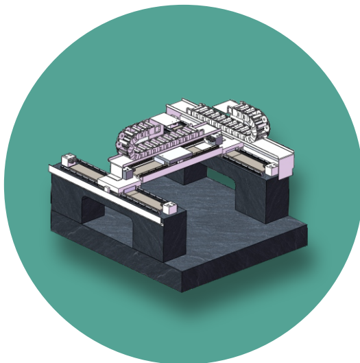
FPC激光切割平臺
